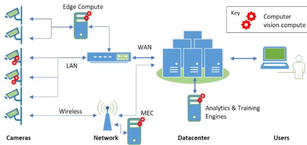
Figure 3: Edge compute
